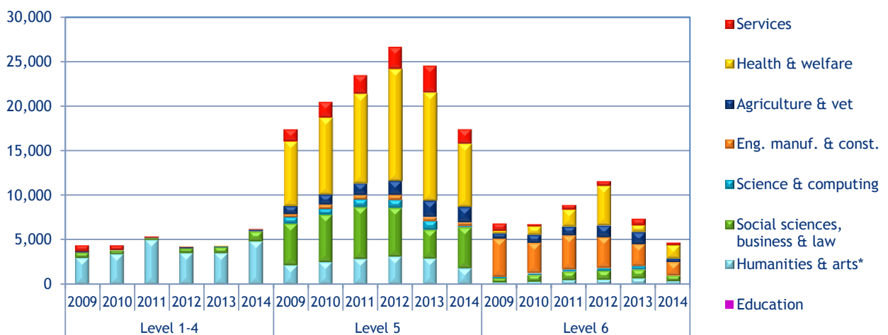
Figure 3.3 QQI (FET) major awards by field of learning, 2009-2014
